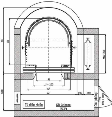
GLASS CABIN LIFT WITH MACHINE ROOM
