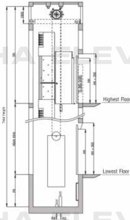
GLASS CABIN LIFT WITHOUT MACHINE ROOM
