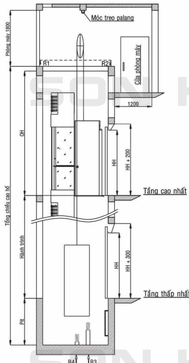
GLASS CABIN LIFT WITH MACHINE ROOM
